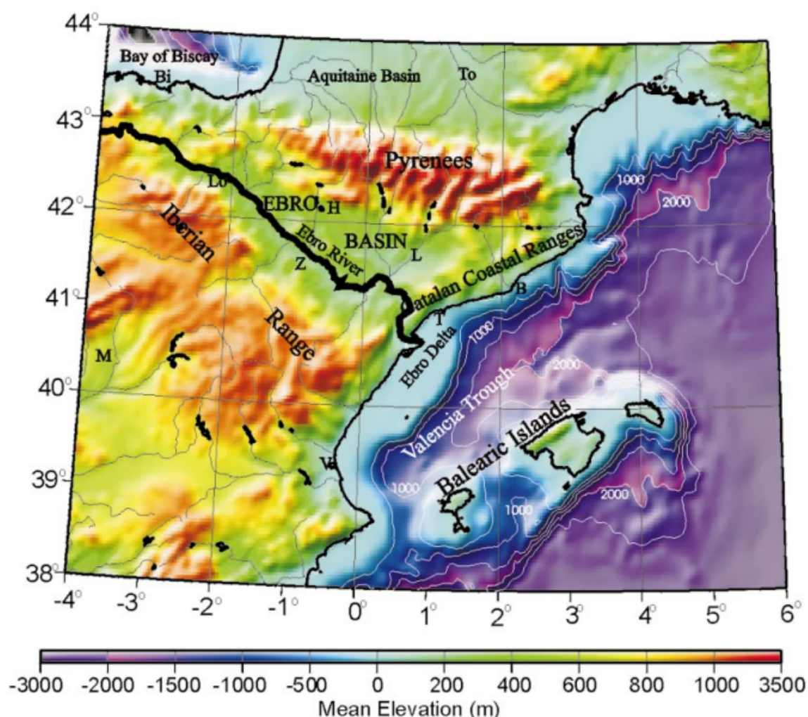
Figure 1. Topographic and bathymetric map of northeastern Iberia and the northwestern Mediterranean, including the main rivers. The Ebro River is highlighted. Note the large prograding shelf-talud of the Ebro Delta. The contour interval of bathymetry is 500 m. B: Barcelona, Bi: Bilbao, H: Huesca, L: Lleida, Lo: Logroño, M: Madrid, T: Tarragona, To: Toulouse, V: Valencia, Z: Zaragoza. Line A-A' refers to Fig. 2.
